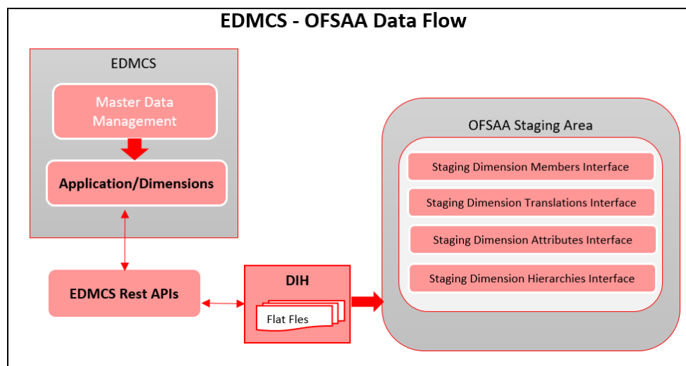
Figure 19: EDMCS - OFSAA Data Flow
